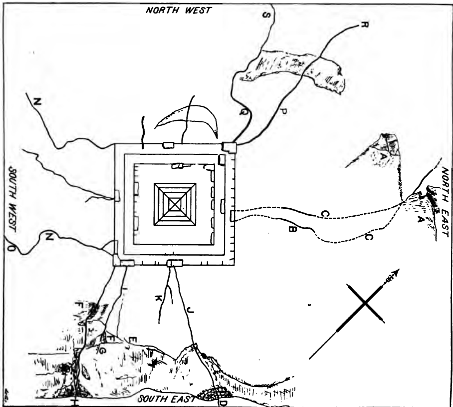
Fig. 4. Ground plan of course of lightning. From "Jour. Met. Soc.," Walker.
